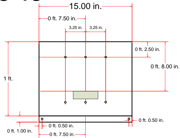
PROJECTOR MOUNT FRONT VIEW
