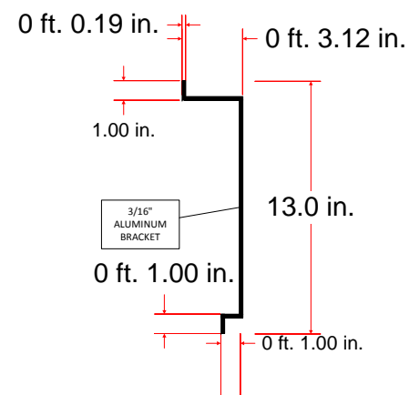
WHITEBOARD MOUNT SIDE VIEW
