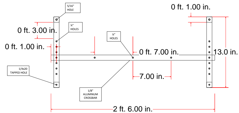
WHITEBOARD MOUNT FRONT VIEW
